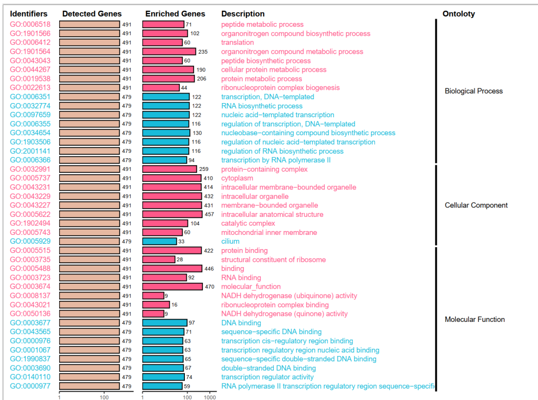
Supplementary Figure 2: Enrichment Analysis of COMMD Scores. (A) KEGG enrichment analysis of COMMD scores. (B) GO enrichment analysis of COMMD scores.
