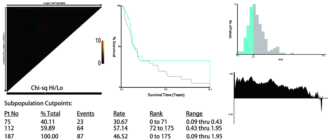
Figure S1 X-tile analyses regarding to OS by using patient data to determine the optimal cut-off value for AAPR. OS: overall survival. AAPR: albumin-to-alkaline phosphatase ratio.
