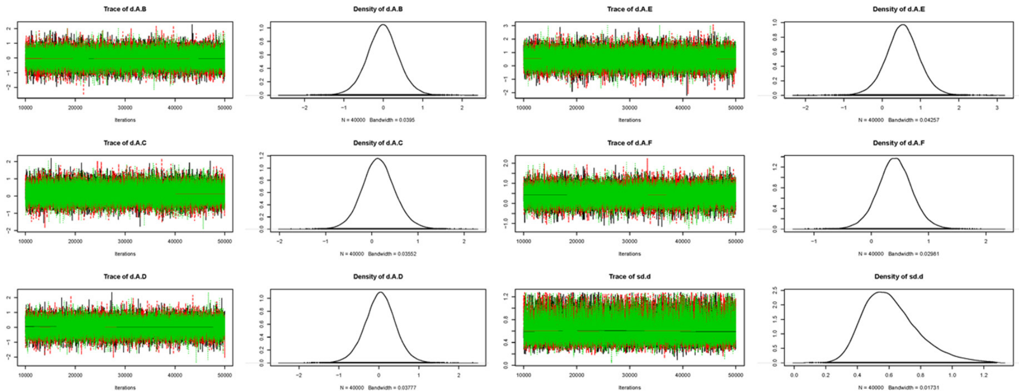
Supplementary Figure 2. Trace plot and density plot. (A) TRUS-GB; (B) TPUS-GB; (C) CEUS; (D) MRI-GB; (E) TRUS+FUS-GB; (F) FUS-GB;
