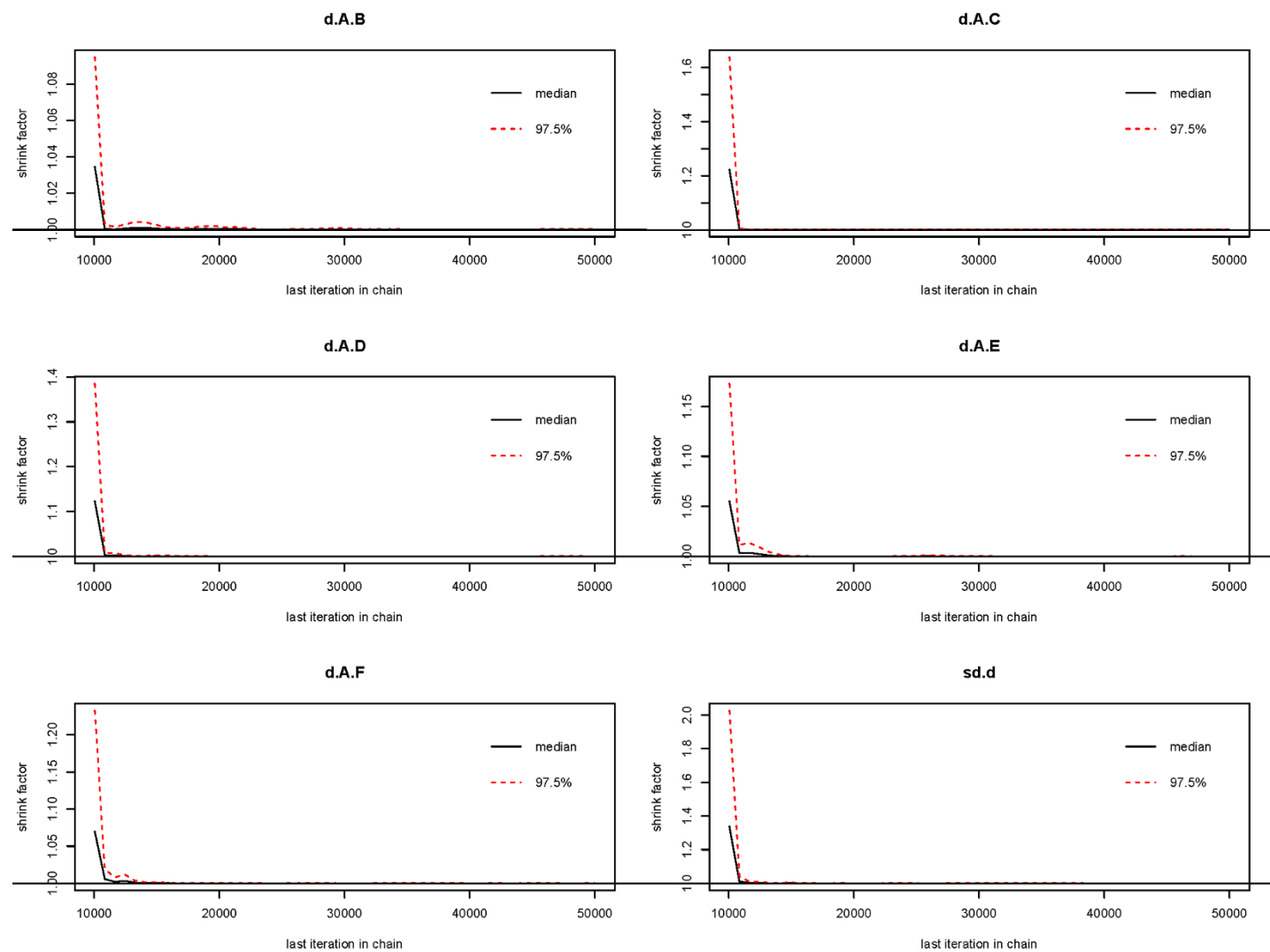
Supplementary Figure 1. Brooks-Gelman-Rubin plots method. (A) TRUS-GB; (B) TPUS-GB; (C) CEUS; (D) MRI-GB; (E) TRUS+FUS-GB; (F) FUS-GB;
